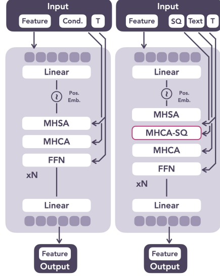
Figure 13: Comparison between the Flow Transformer from the original Trellis ( left ) and the one from SPICE-E-T ( right ), adapted to enable spatial control via superquadrics.
